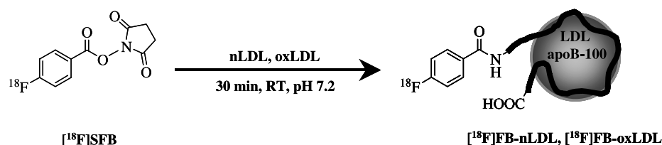
Fig. 1. Proposed reaction scheme of selective [ ^{18}\text{F} ]fluorobenzoylation of LDL apoB-100 at its chemically accessible glutamate amino-terminal residue at pH 7.2
